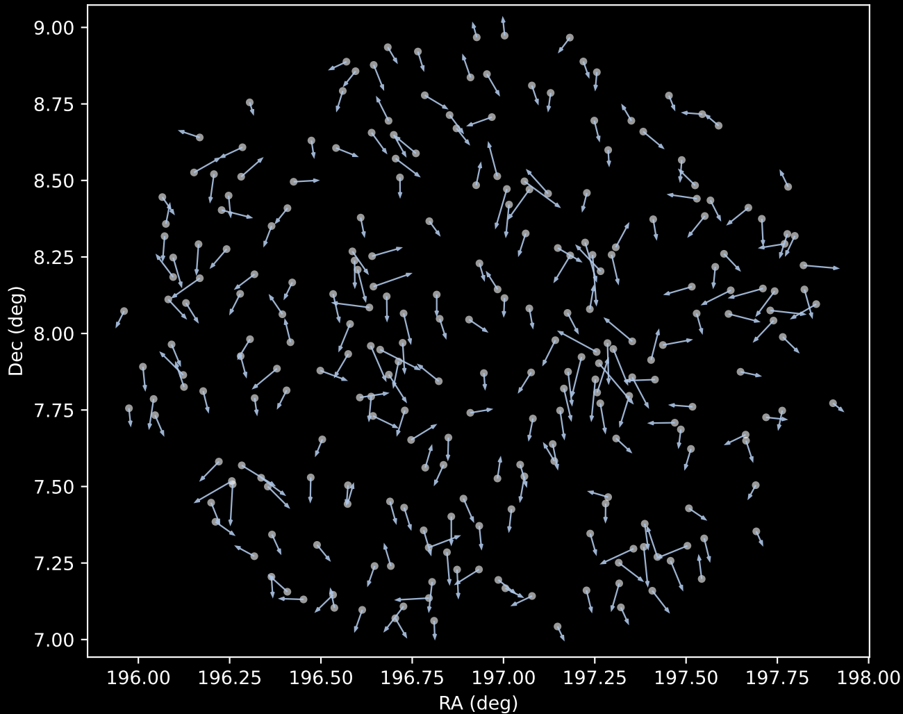
GALAH DR4 Cluster 1 Proper Motion Vectors (n=253)
