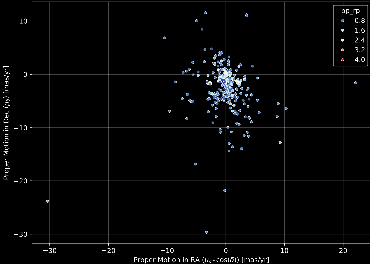
GALAH DR4 Field: [9471] Proper Motion Diagram (n= 276)
