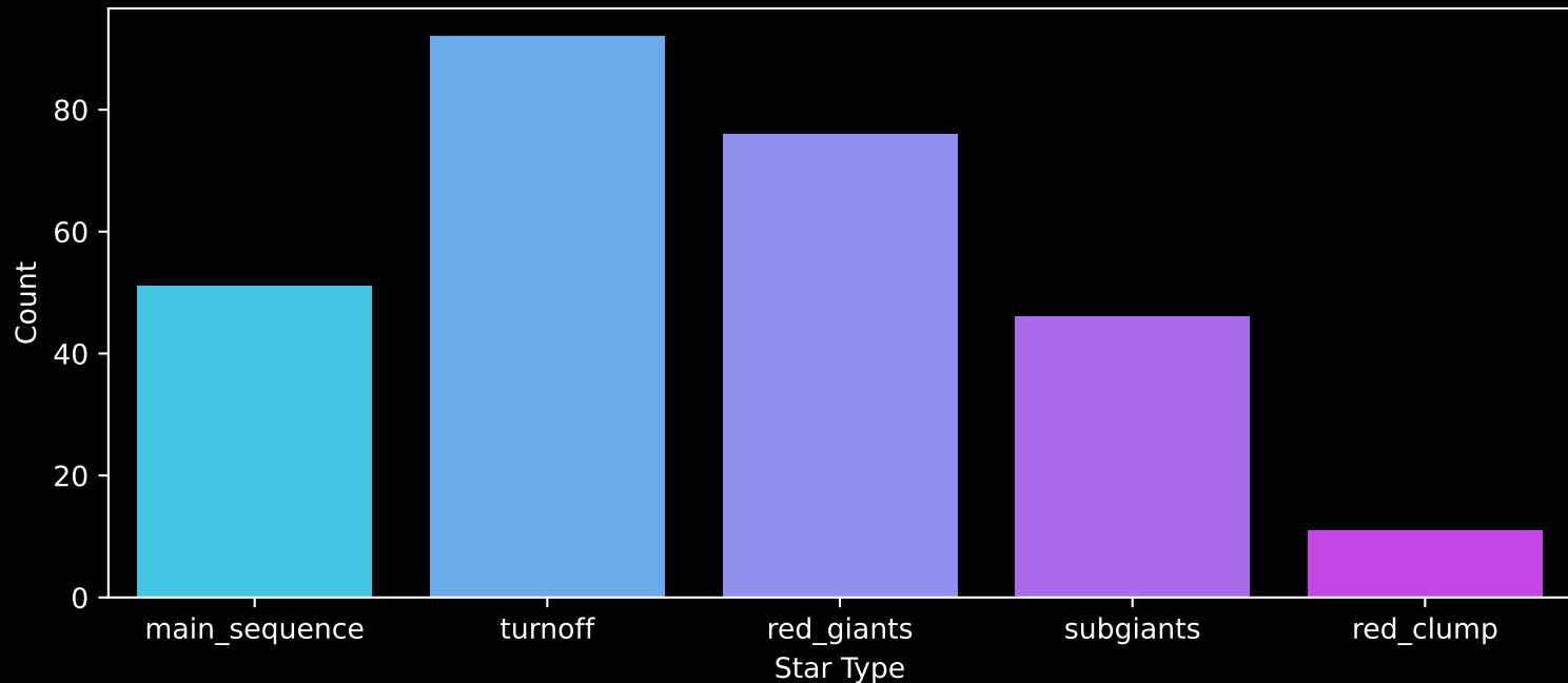
GALAH DR4 Field: [9471] Count plot of Star Type
