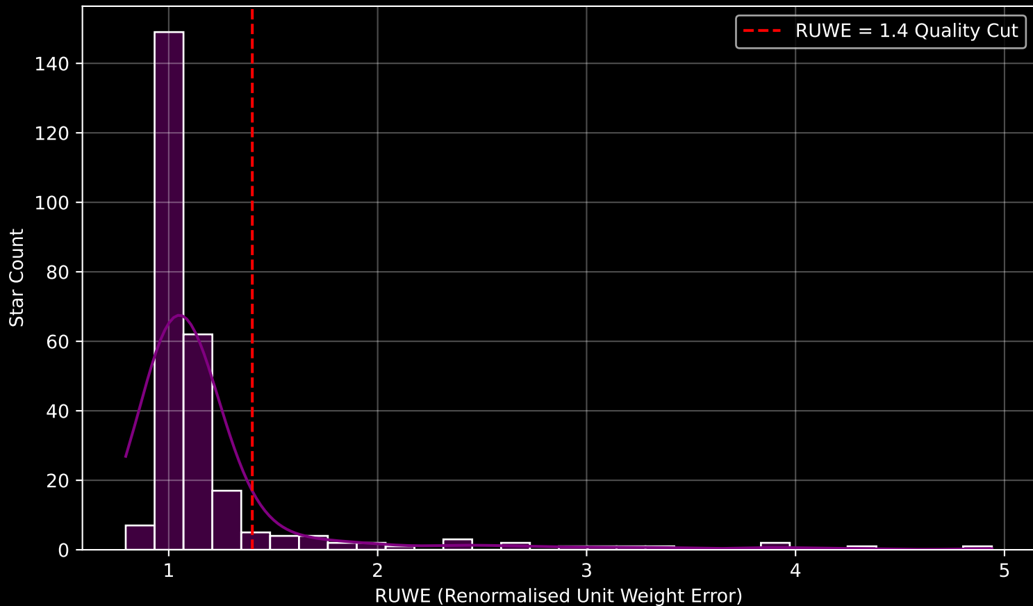
GALAH DR4 Field [9471] RUWE Distribution (n= 266)
